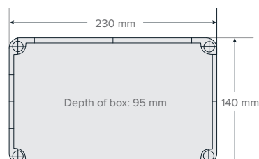
A12 Power Box – Fixed Colour/Multicoloured RGBW
